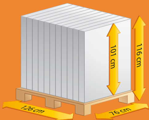
Optilook access roof light 46 x 75 Quantity per pallet – 11 pcs.
